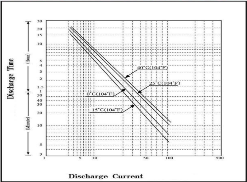
Discharge Characteristics(0°C/32°F,40°C/104°F)
