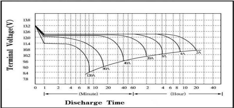
Discharge Characteristics(20°C,68°F)
